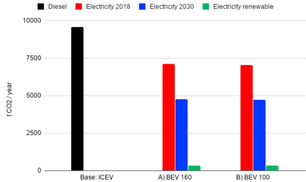
Fig. 2. Calculated CO2 emissions per year.
