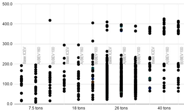
Fig. 1. Observed daily tour distances [km] driven by vehicle type and case.
